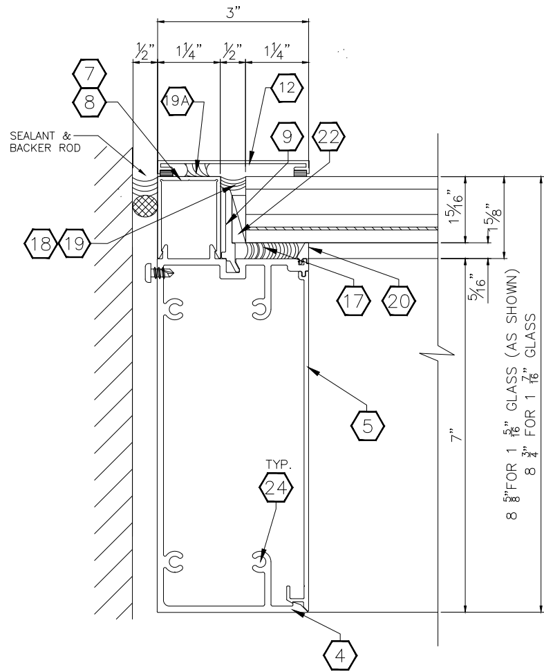
1 HEAD DETAIL 12 W/ EXTERIOR COVER
