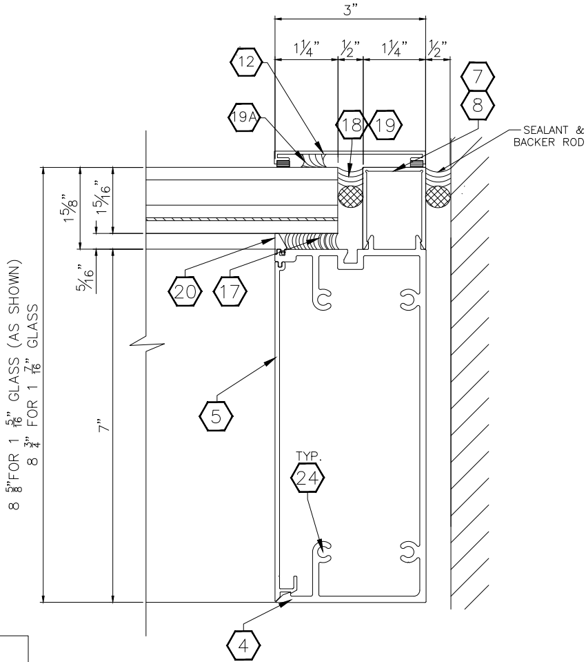
3 SILL DETAIL 12 W/ EXTERIOR COVER
