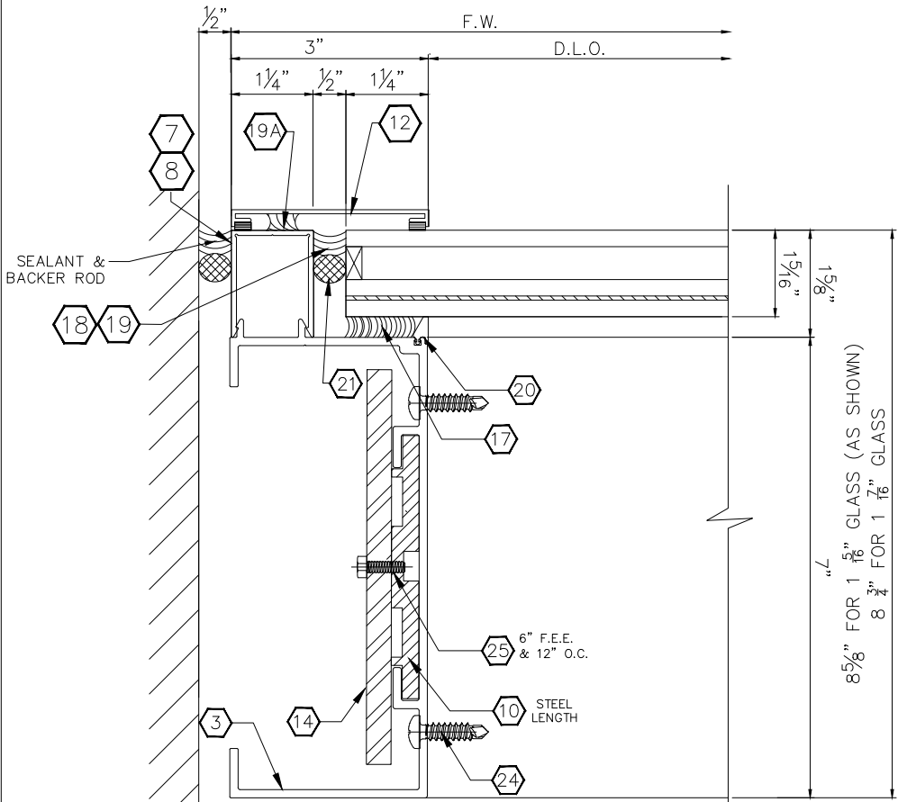
4 JAMB DETAIL 12 W/ EXTERIOR COVER
