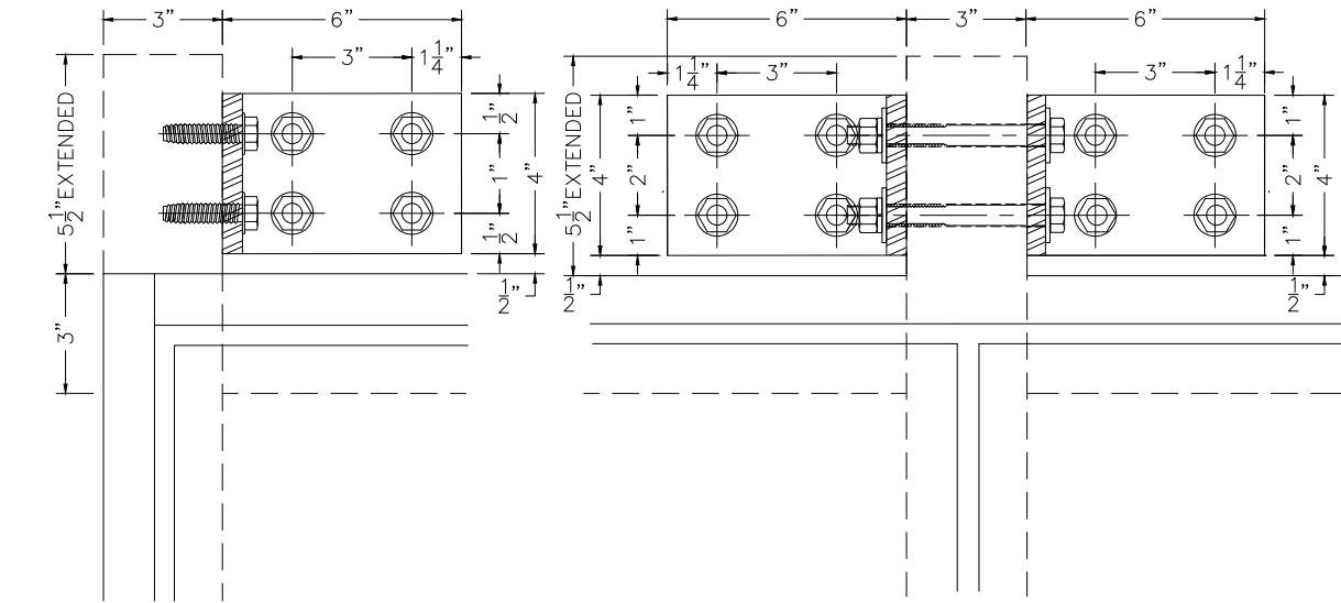
HEAD/SILL(OPP.) ANCHOR TYPE A IN WOOD ANCHOR TYPE B IN ALUMINUM OR STEEL (4) AT JAMB INT. VERTICAL ANCHOR TYPE A IN WOOD ANCHOR TYPE B IN ALUMINUM OR STEEL (8) AT VERTICAL
