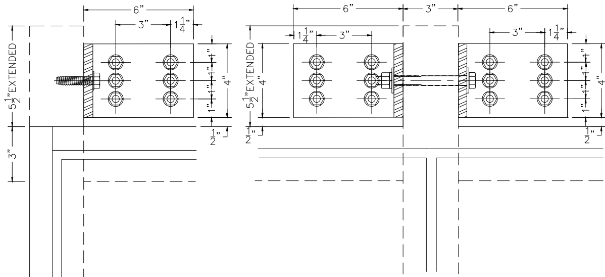
HEAD/SILL(OPP.) ANCHOR TYPE A IN WOOD (6) AT JAMB OR (5) AT JAMB INT. VERTICAL ANCHOR TYPE A (12) AT VERTICAL OR (10) AT VERTICAL
