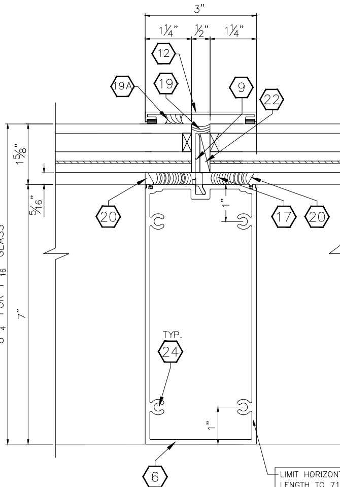
2 INT. HORIZONTAL DETAIL 12 W/ EXTERIOR COVER
