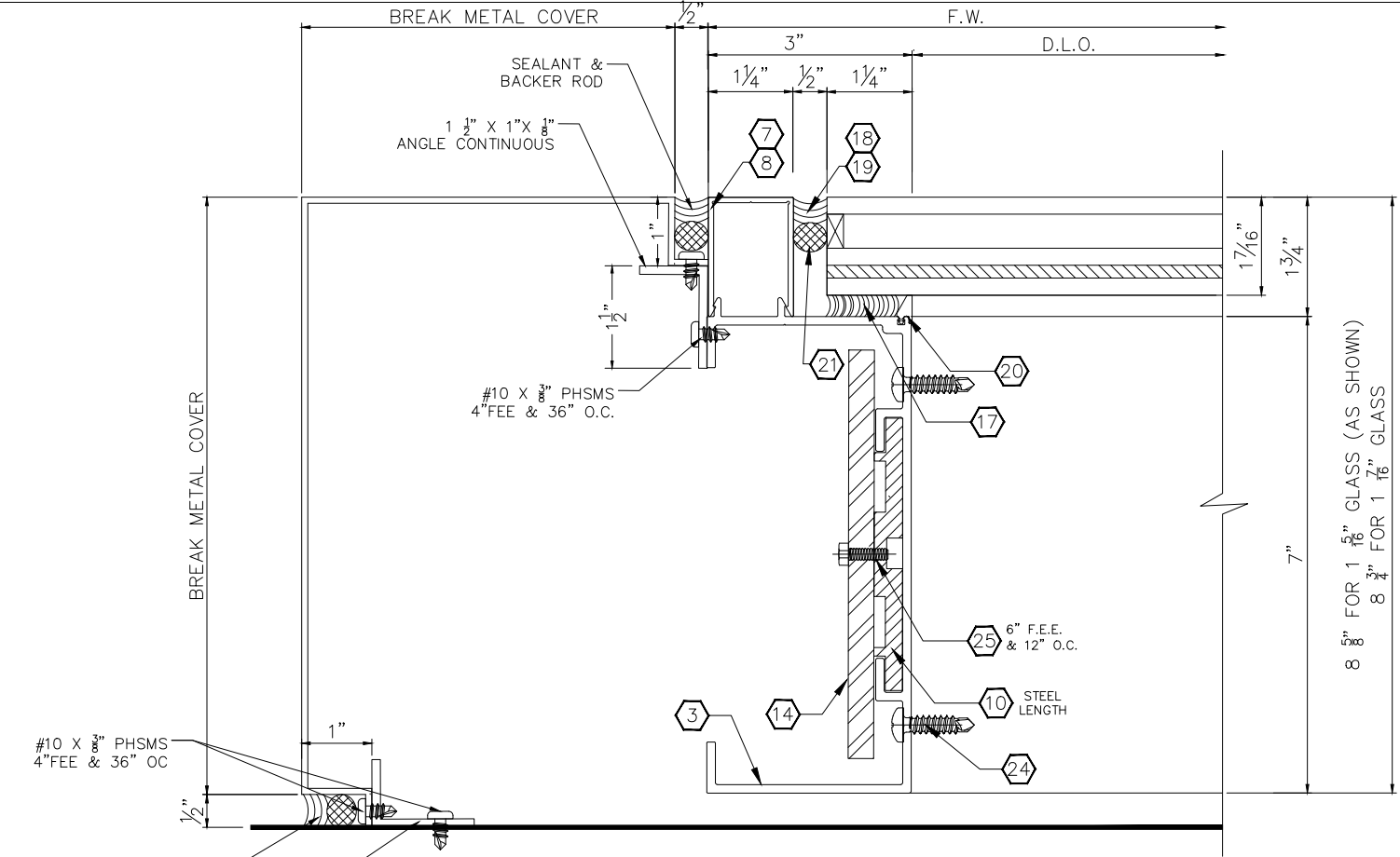
1 REINFORCED JAMB DETAIL 8 W/ STEEL REINFORCEMENT TYPE 1 3/8" X 6" FLAT BAR STL. LENGTH = MULL. LENGTH
