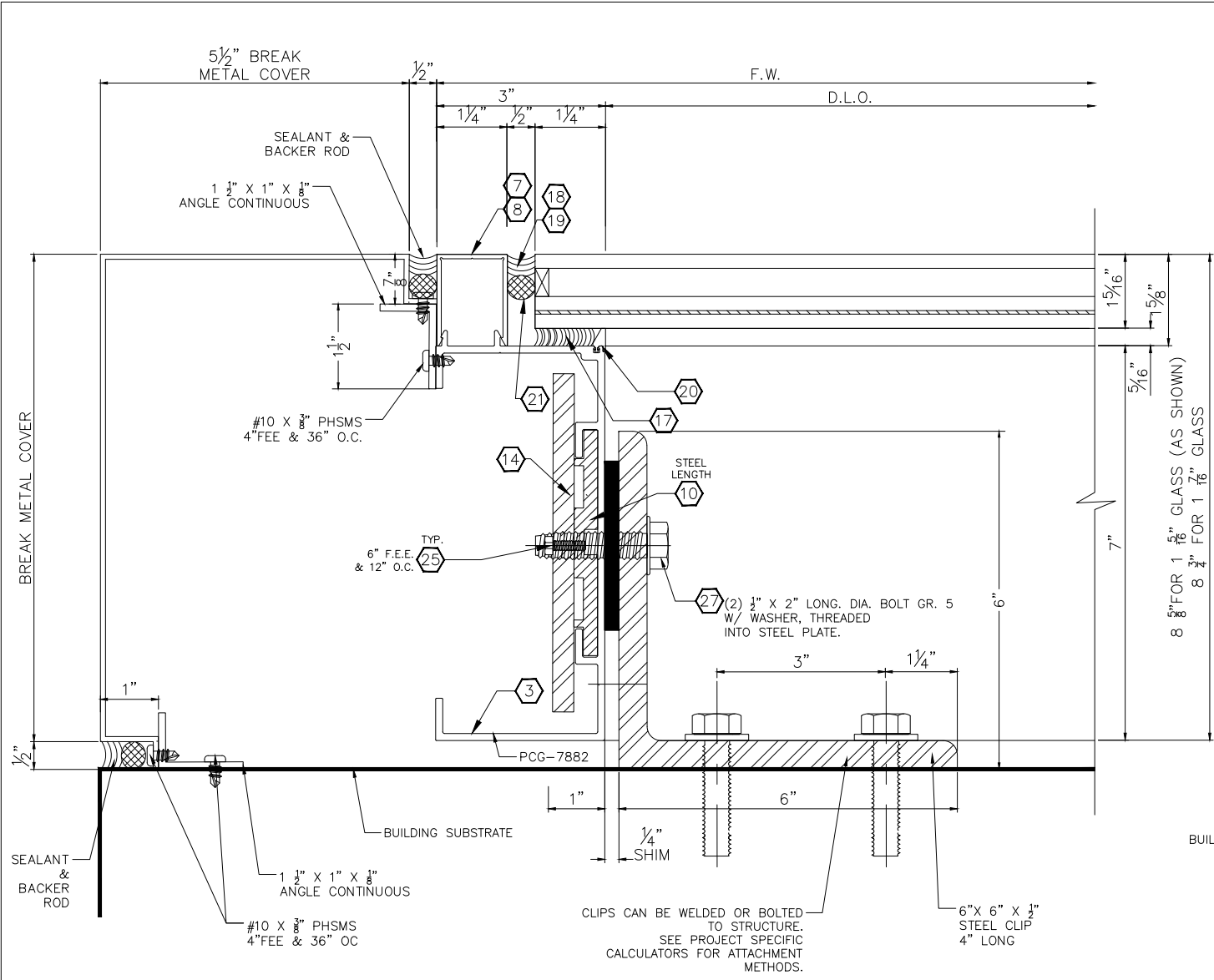
1 JAMB DETAIL ANCHOR 11
