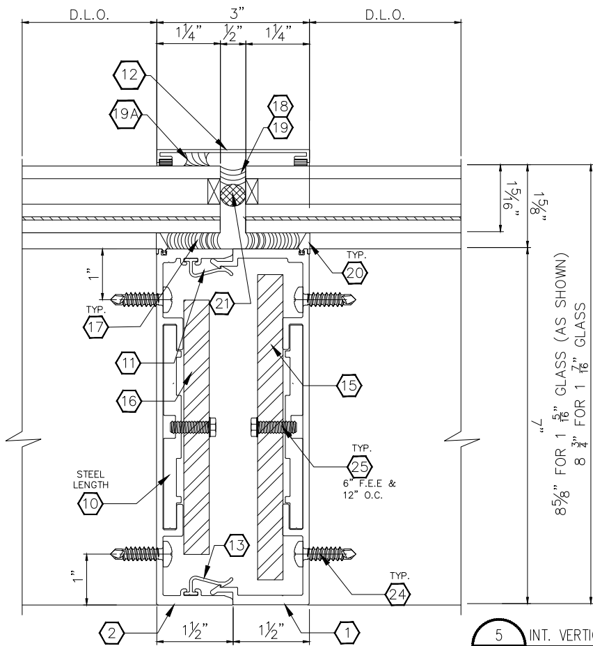
2 INT. HORIZONTAL DETAIL 12 W/ EXTERIOR COVER
