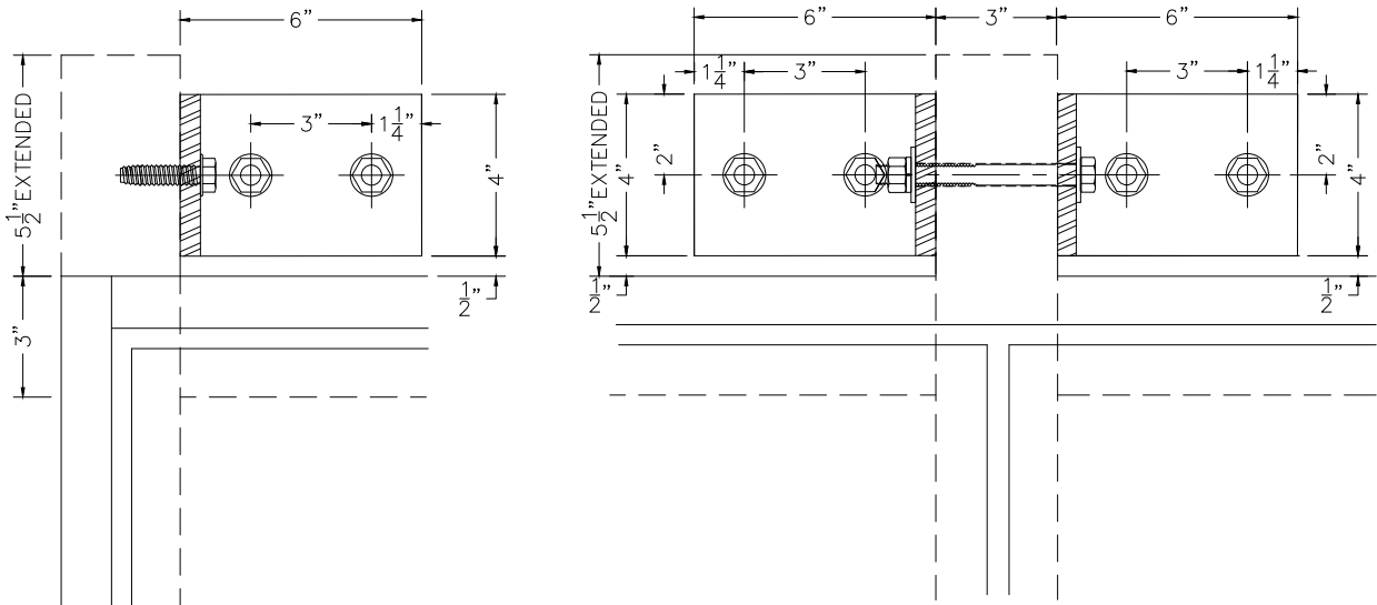
HEAD/SILL(OPP.) ANCHOR B1 IN ALUMINUM OR STEEL ANCHOR TYPE C IN CONCRETE (2) AT JAMB INT. VERTICAL ANCHOR B1 IN ALUMINUM OR STEEL ANCHOR TYPE C IN CONCRETE (4) AT VERTICAL
