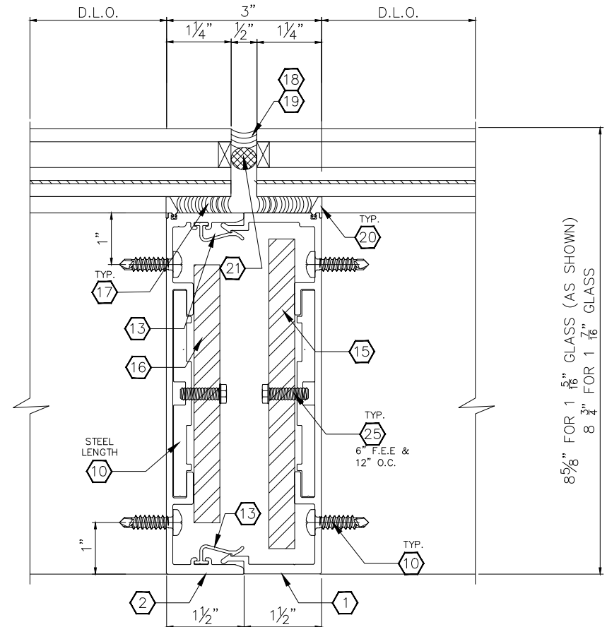
2 INT. VERTICAL MULLION DETAIL 8 W/ STEEL REINFORCEMENT TYPE 2 & 3 1/2"X5" & 1/2"X 6" STEEL FLAT BAR STL. LENGTH = MULL. LENGTH
